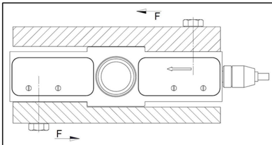
Figure 2: Installation conditions
